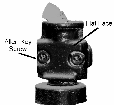
Flat Style Inlet with Flat Face And Allen Key Screws HOMA Part Number Or Pump Serial Number Must Be Supplied With This Model
